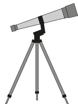
telescoop
